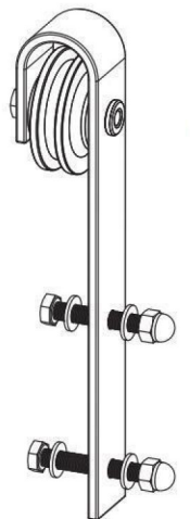
Hangers x2
